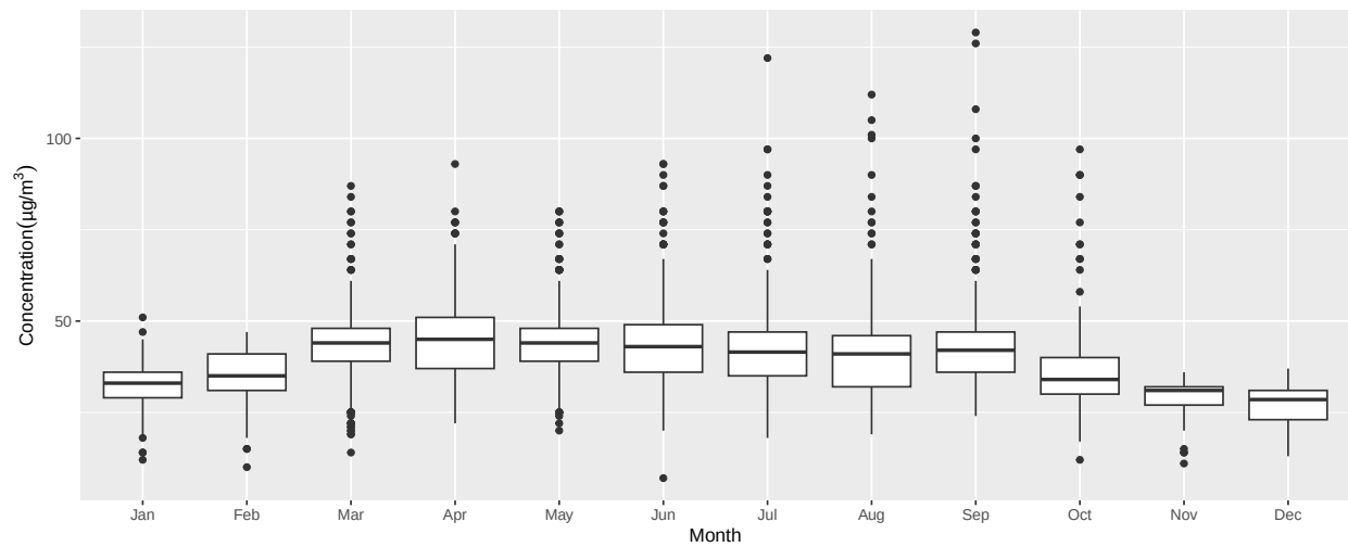
Figure 2: 2019 monthly Ozone levels
