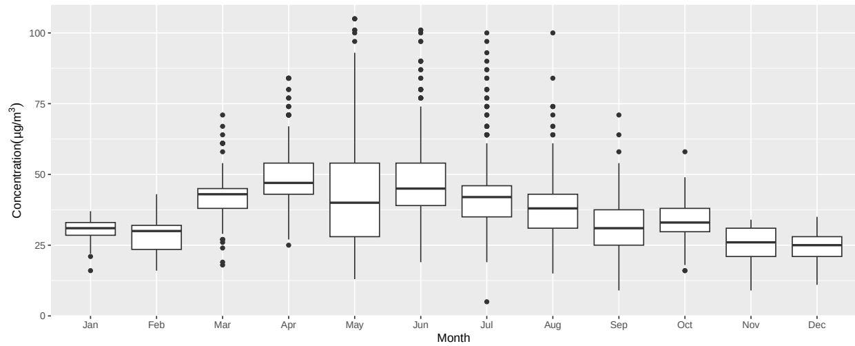
Figure 1: 2018 monthly Ozone levels
